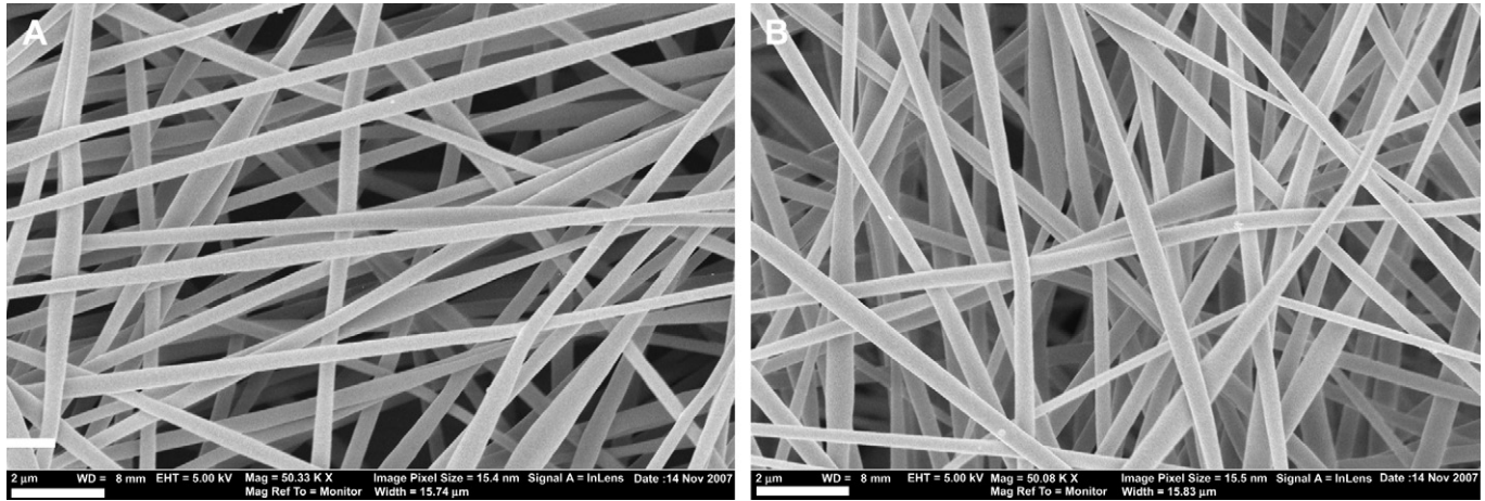
Fig. 1. SEM micrographs of electrospun silk fibroin scaffolds: (A) PEO non-extracted scaffold; (B) PEO extracted scaffold. Scale bars are 2 \mu\text{m} .
