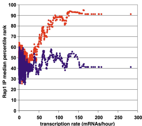
Fig. 4 Rap1 binds to the promoters of heavily transcribed genes. The median percentile rank of enrichment detected by the arrayed intergenic segment immediately upstream of each yeast ORF in Rap1 IPs (red, moving median; window size=20) or control IPs (blue), plotted as a function of the transcription rate (mRNAs/hour) of that ORF 29 . All ORFs are plotted.
